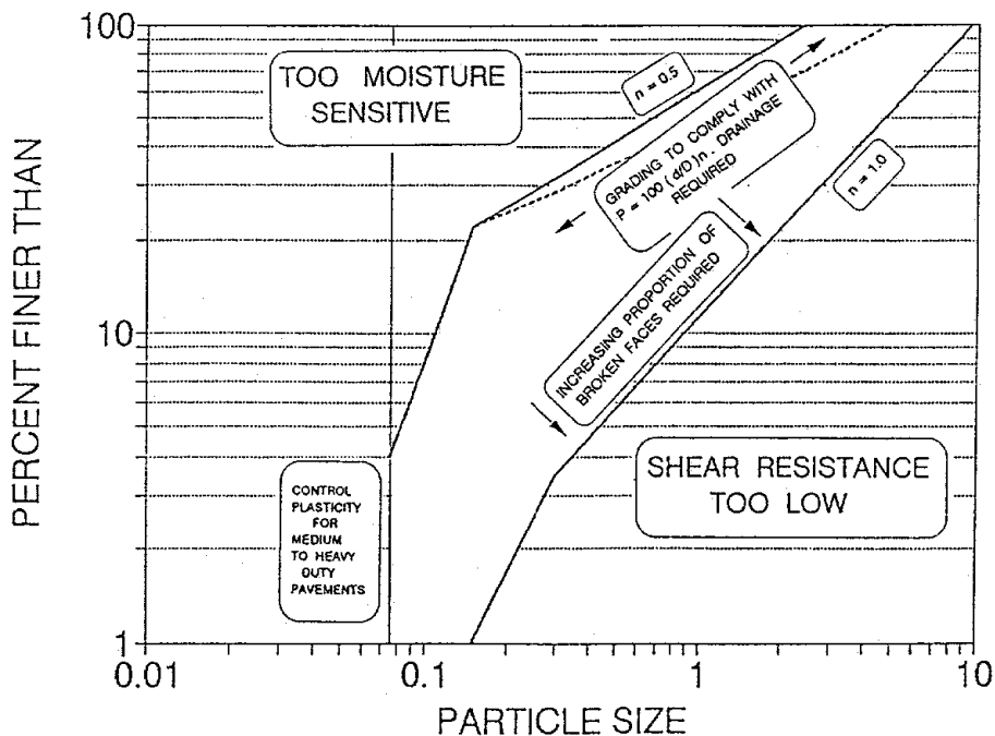
FIGURE 2 PROPOSED GRADINGS FOR BEDDING MATERIALS
