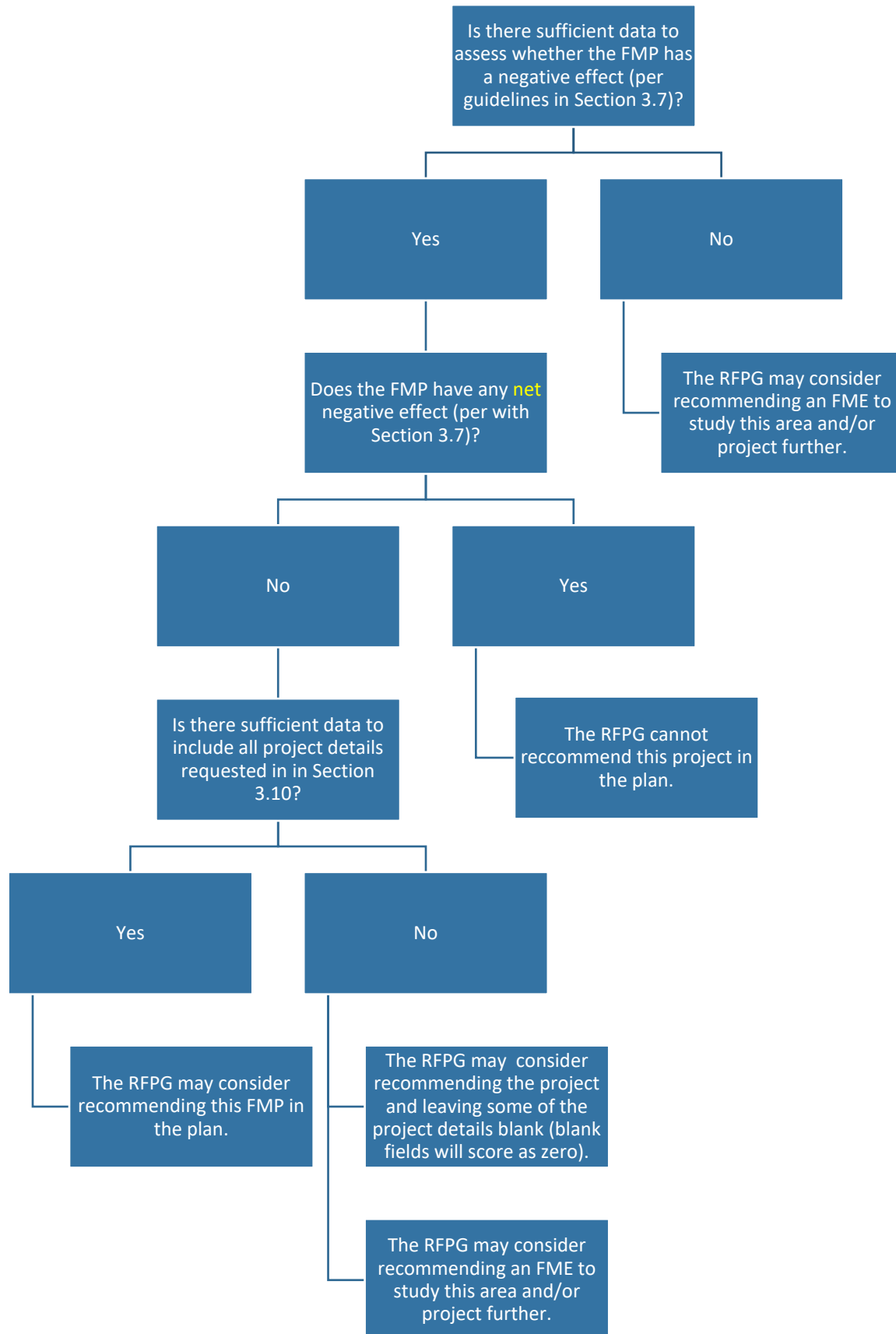
Figure 5: FMP flowchart
