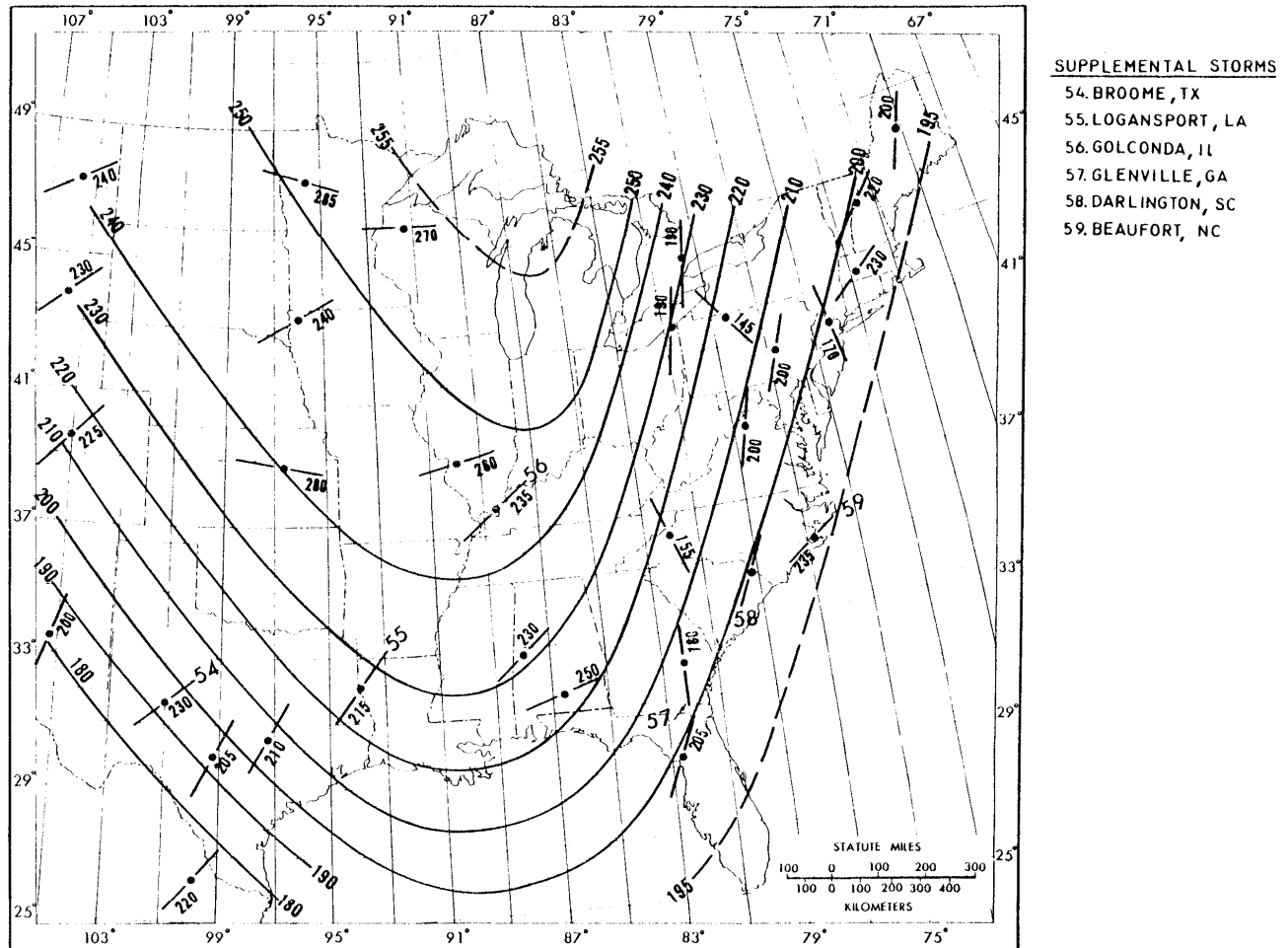
Figure 8.--Analysis of isohyetal orientations for selected major storms adopted as recommended orientation for HMP within \pm 40^\circ . Addition of 6 major storms not in figure 7 have been identified numerically above station locations and in the margin.
