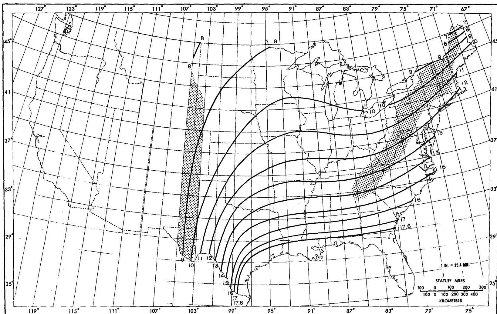
Figure 40.--All-season PMP (in.) for 24 hr 10,000 mi 2 (25,900 km 2 ).
