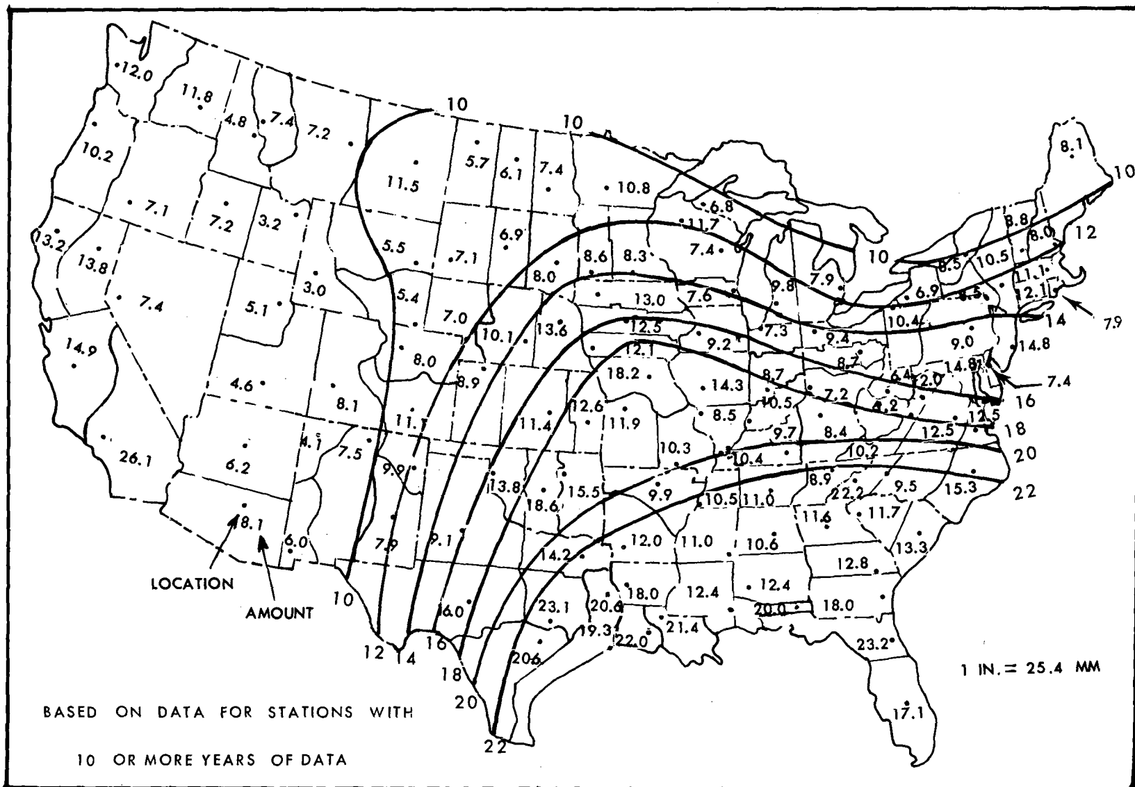
Figure 9.--Envelopment of the greatest 24-hr station precipitation (in.) within each State climatic division (through 1970).
