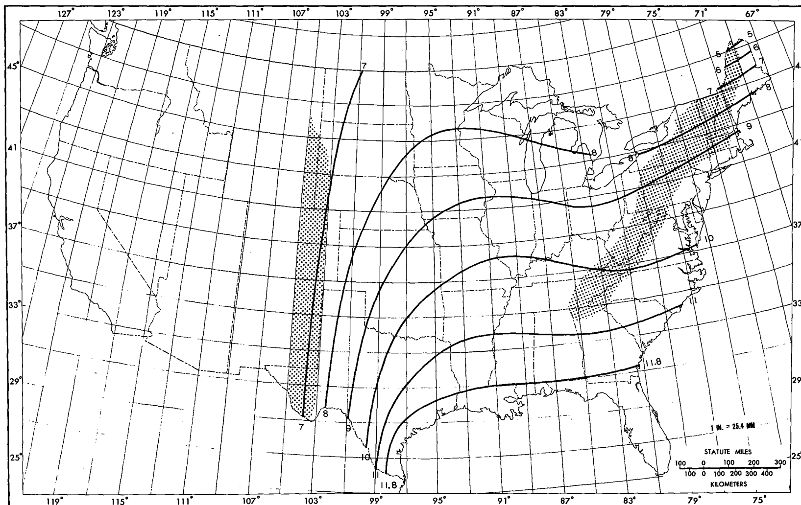
Figure 39.--All-season PMP (in.) for 12 hr 10,000 mi 2 (25,900 km 2 ).
