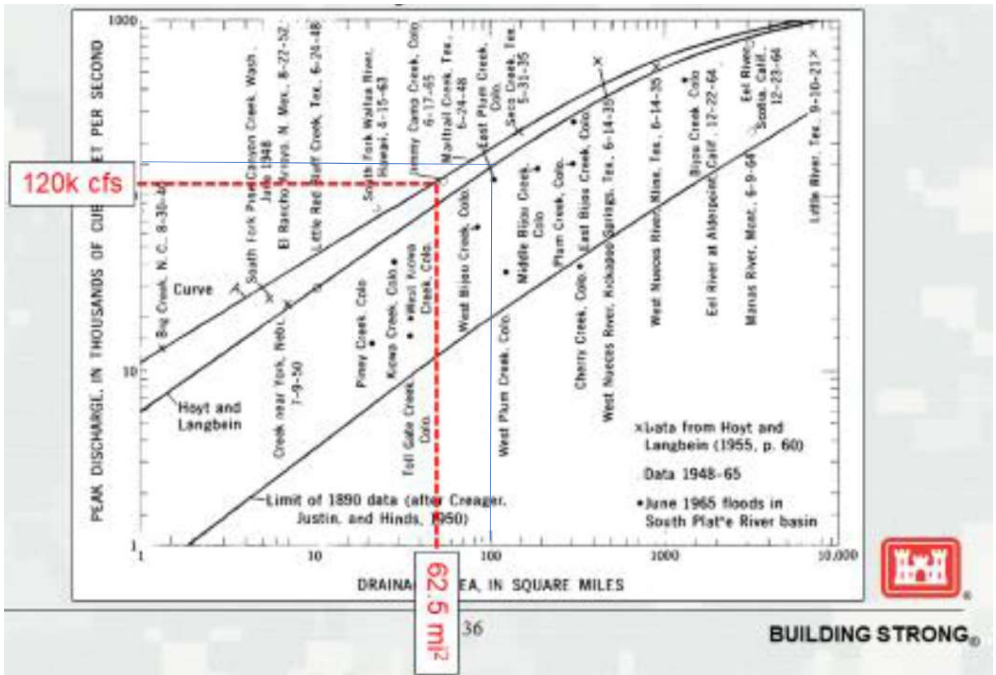
Peak Discharge ( 10^3 cfs) vs. Drainage Area (Sq Mi)
