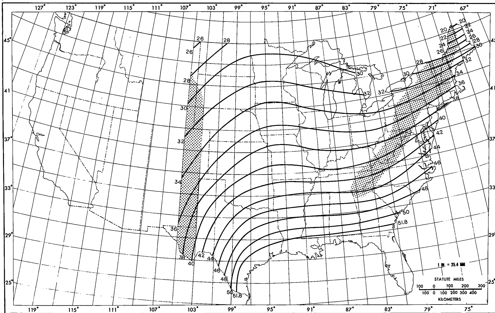
Figure 21.--All-season PMP (in.) for 48 hr 10 mi 2 (26 km 2 ).
