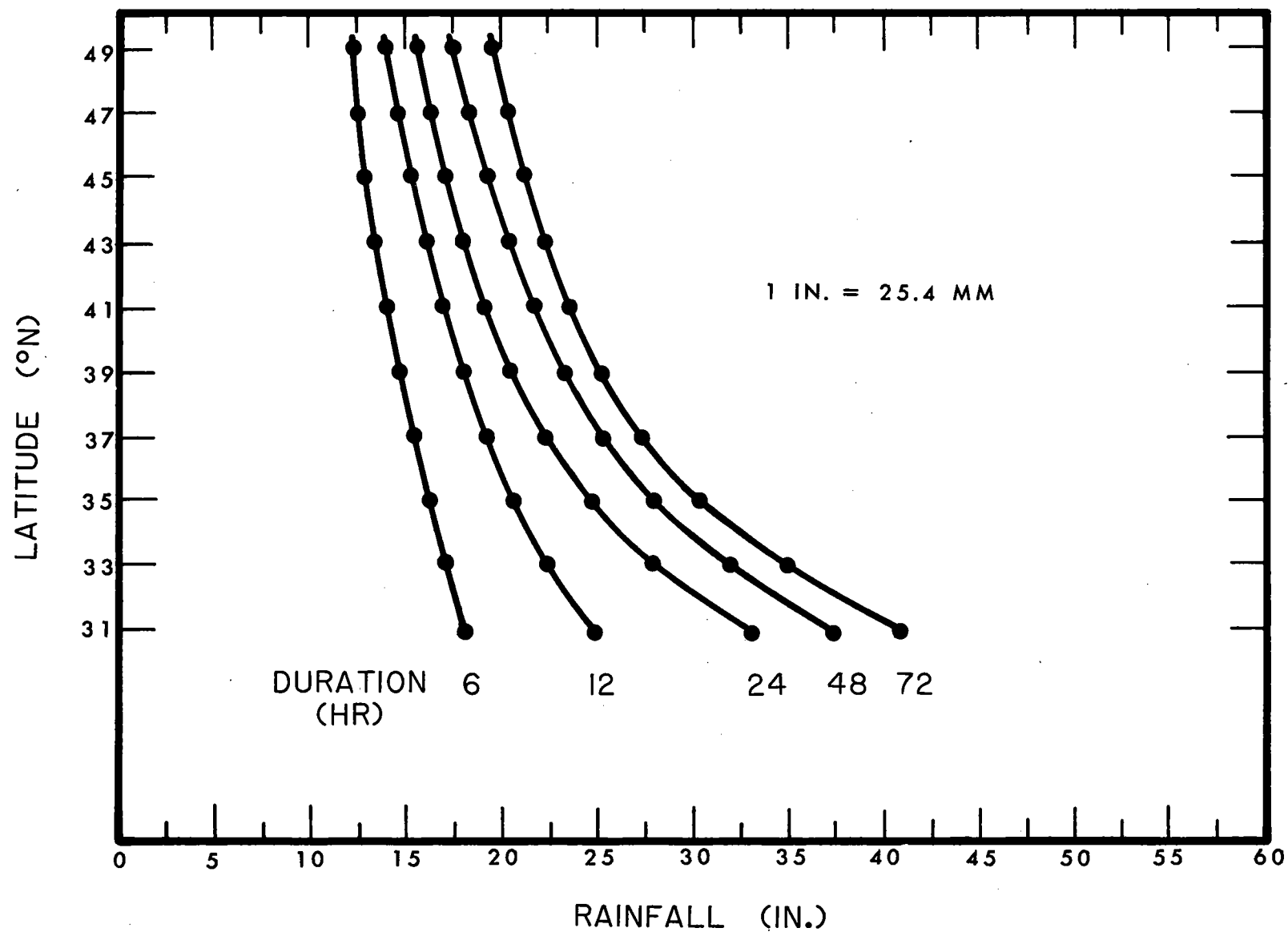
Figure 15.--Example of cross-section smoothing--constant area. [Depth vs. latitude along 91°W longitude for 1,000 mi 2 (2,590 km 2 ) ]
