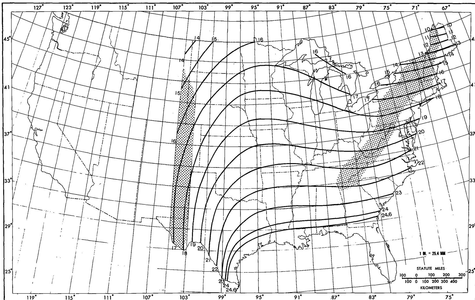
Figure 23.--All-season PMP (in.) for 6 hr 200 mi 2 (518 km 2 ).
