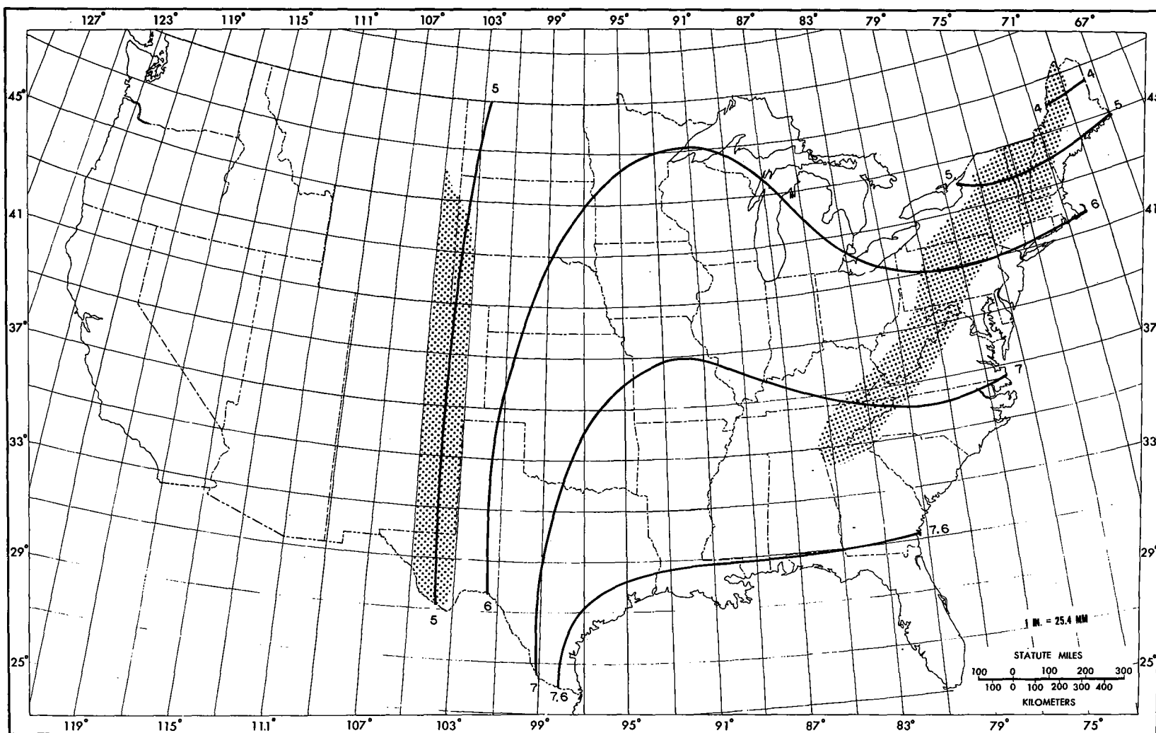
Figure 38.--All-season PMP (in.) for 6 hr 10,000 mi 2 (25,900 km 2 ).
