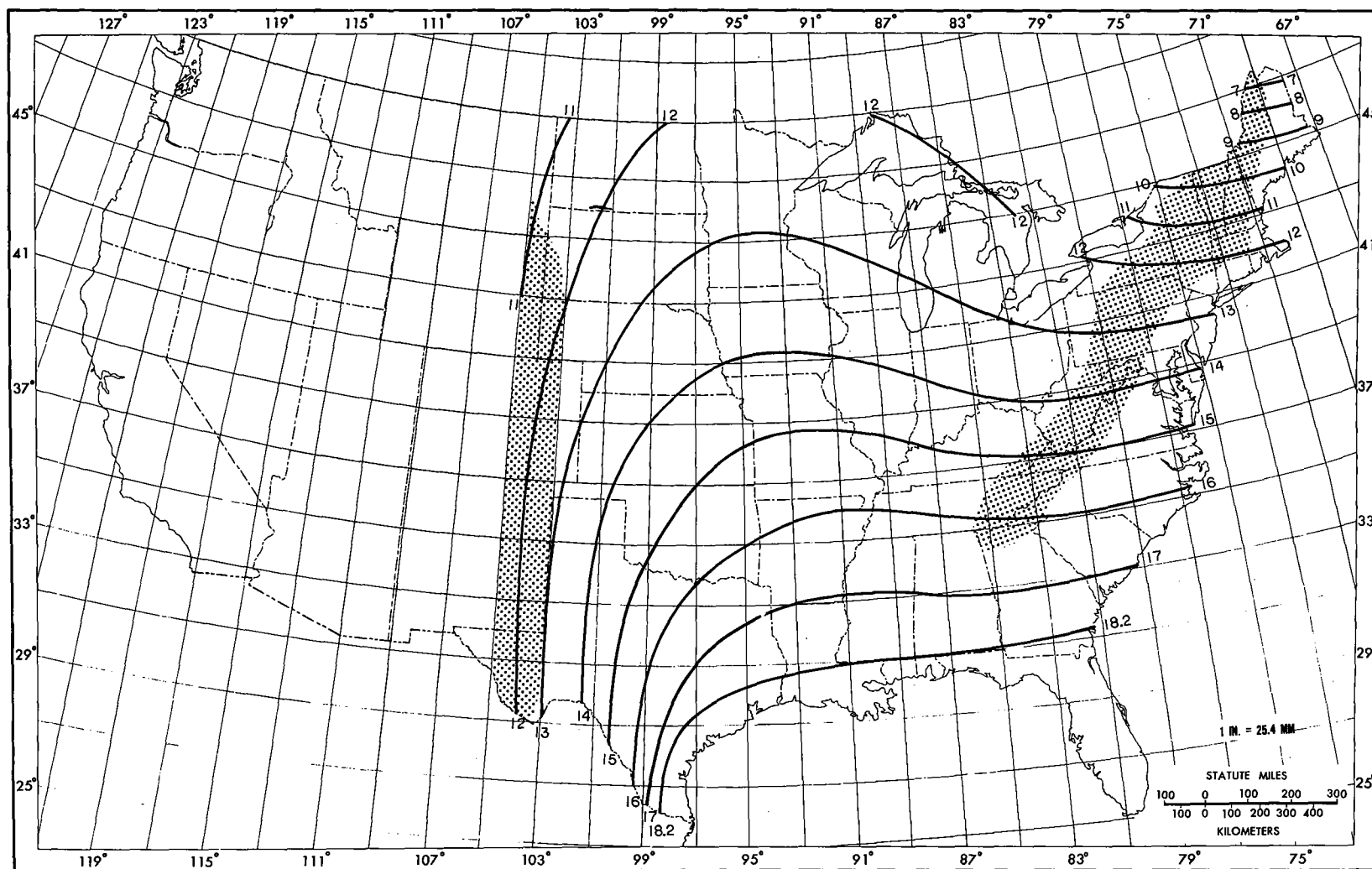
Figure 28.--All-season PMP (in.) for 6 hr 1,000 mi 2 (2,590 km 2 ).
