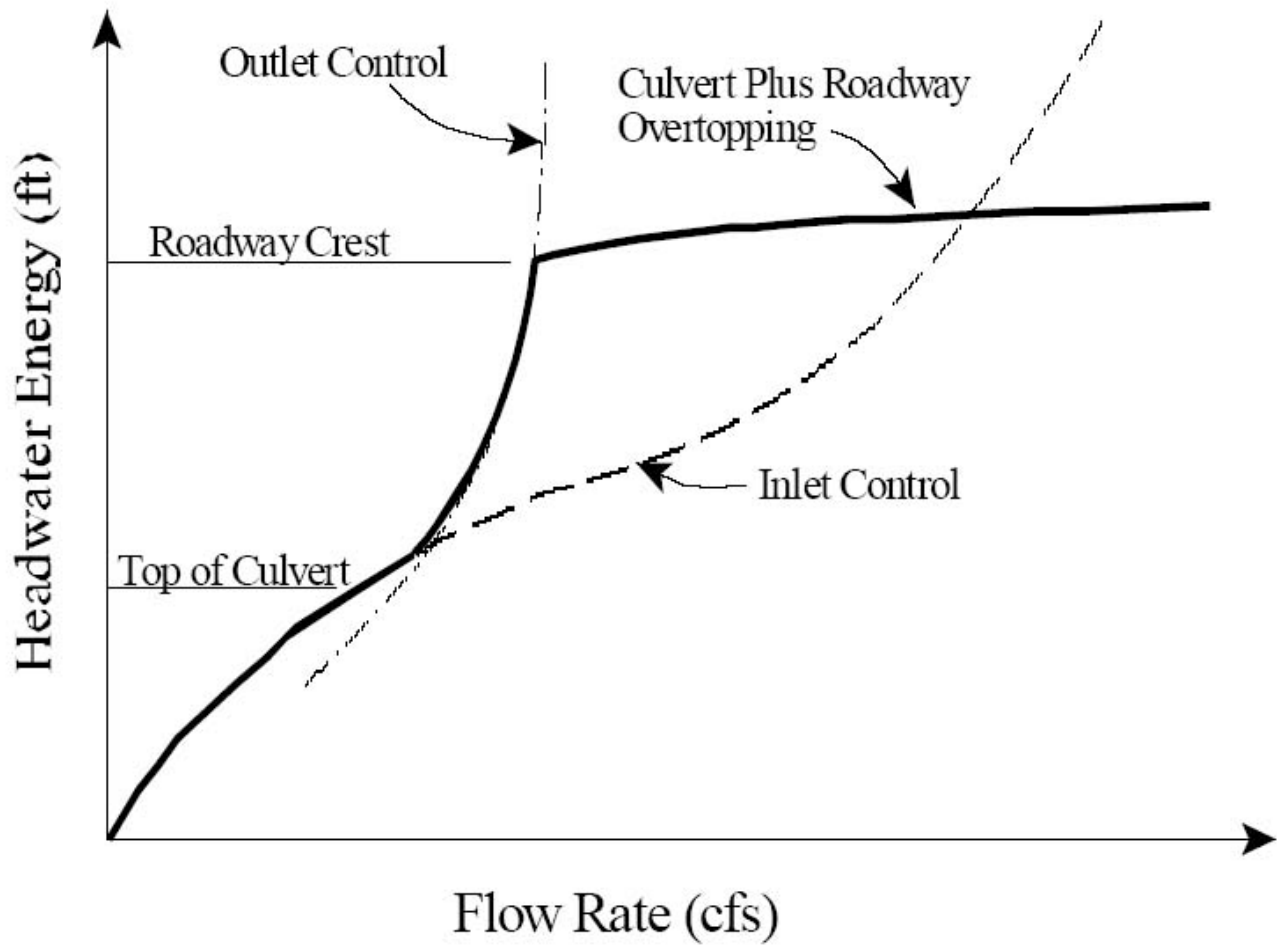
Figure 6.8 Culvert performance curve with roadway overtopping.
