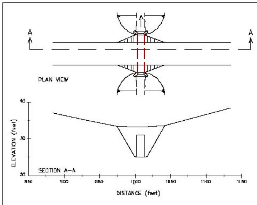
Figure 6.1 Typical culvert road crossing.
