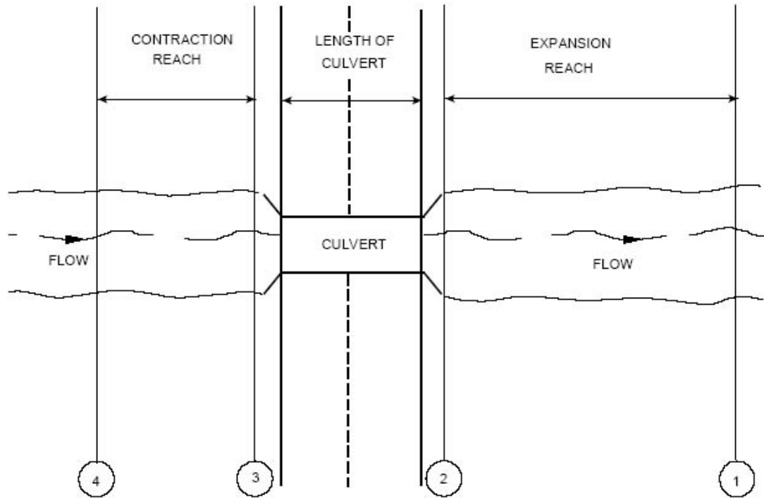
Figure 6.3 Cross section layout for culvert method.
