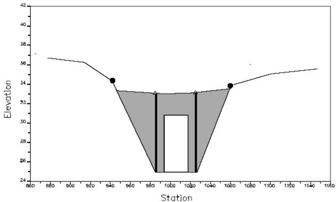
Figure 6.5 Cross section 3 of culvert model.
