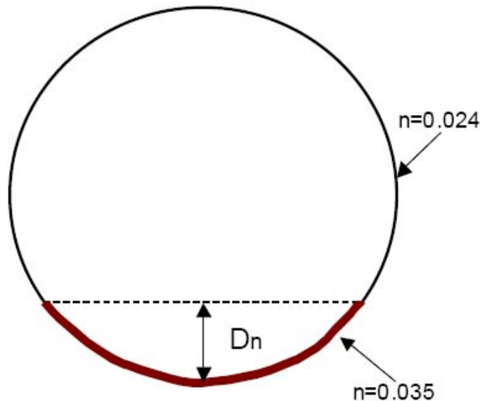
Figure 6.10 Culvert with multiple Manning's n values.
