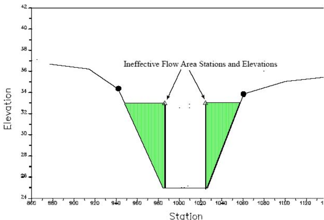
Figure 6.4 Cross section 2 of culvert model.
