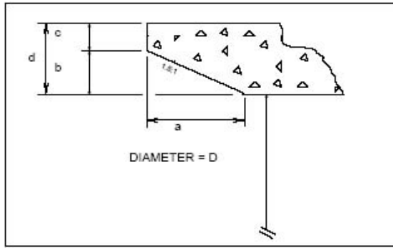
Figure 6.17 Culvert Inlet with Beveled Ring Entrance.
