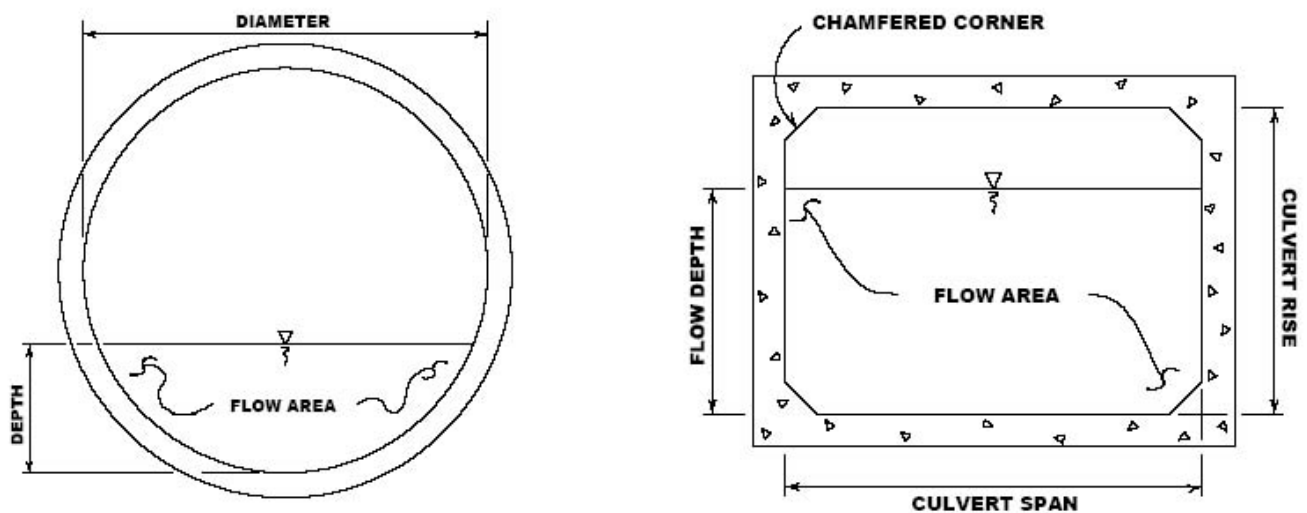
Figure 6.6 Cross section of a circular pipe and box culvert, respectively.
