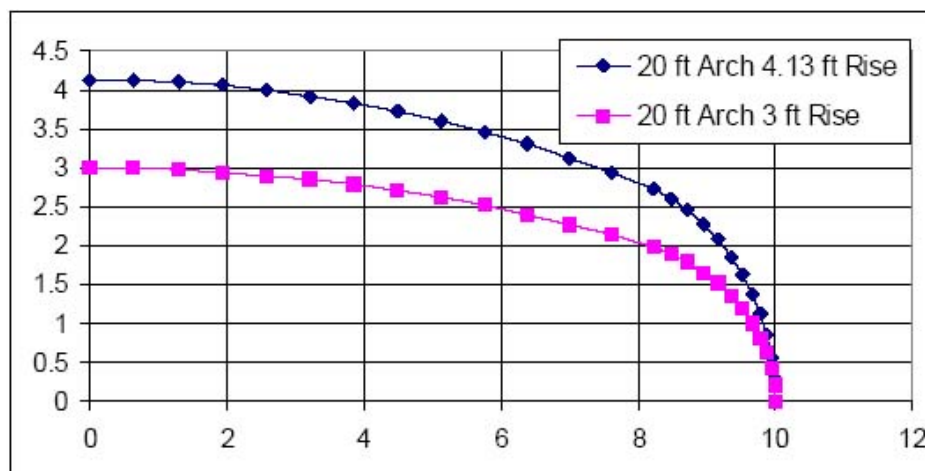
Figure 6.13 Geometric Interpolation of the ConSpan Culvert for Non-Standard Rise.
