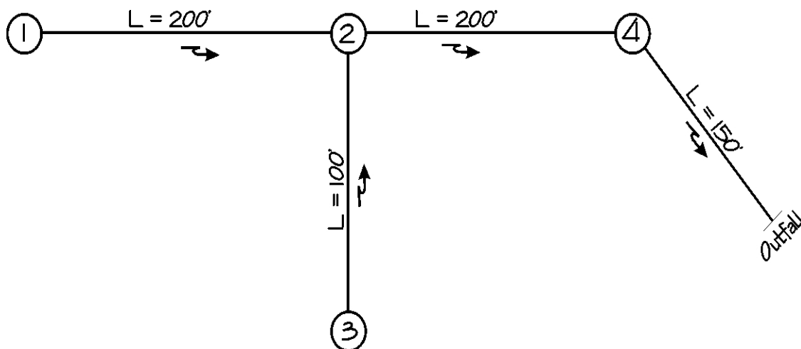
Figure 9-10* Storm Drain Layout Sample Problem
