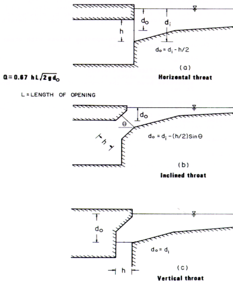
Figure 9-6 Curb Opening Inlets (Operating as an Orifice)
