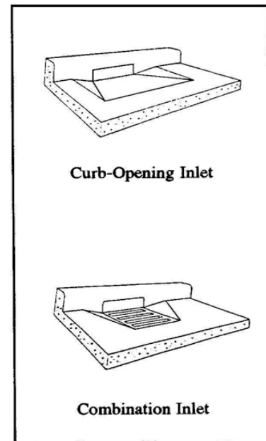
Figure 9-3 Curb Inlets
