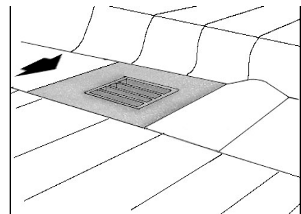
Figure 9-5 Grate Inlets
