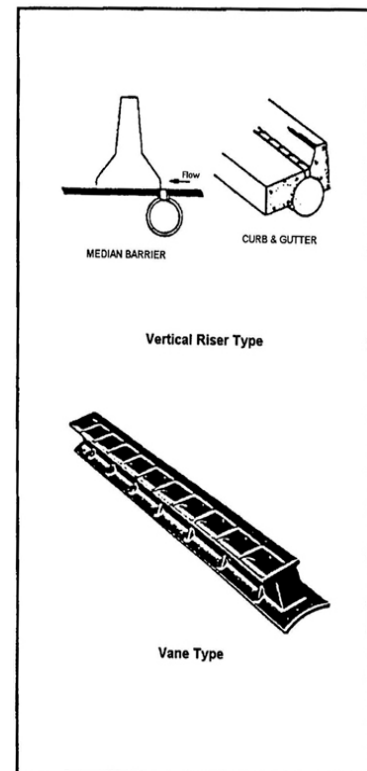
Figure 9-4 Slotted Drain Inlets
